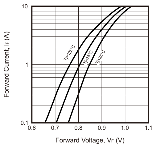
Fig.3 - Typical Forward Voltage Characteristic
